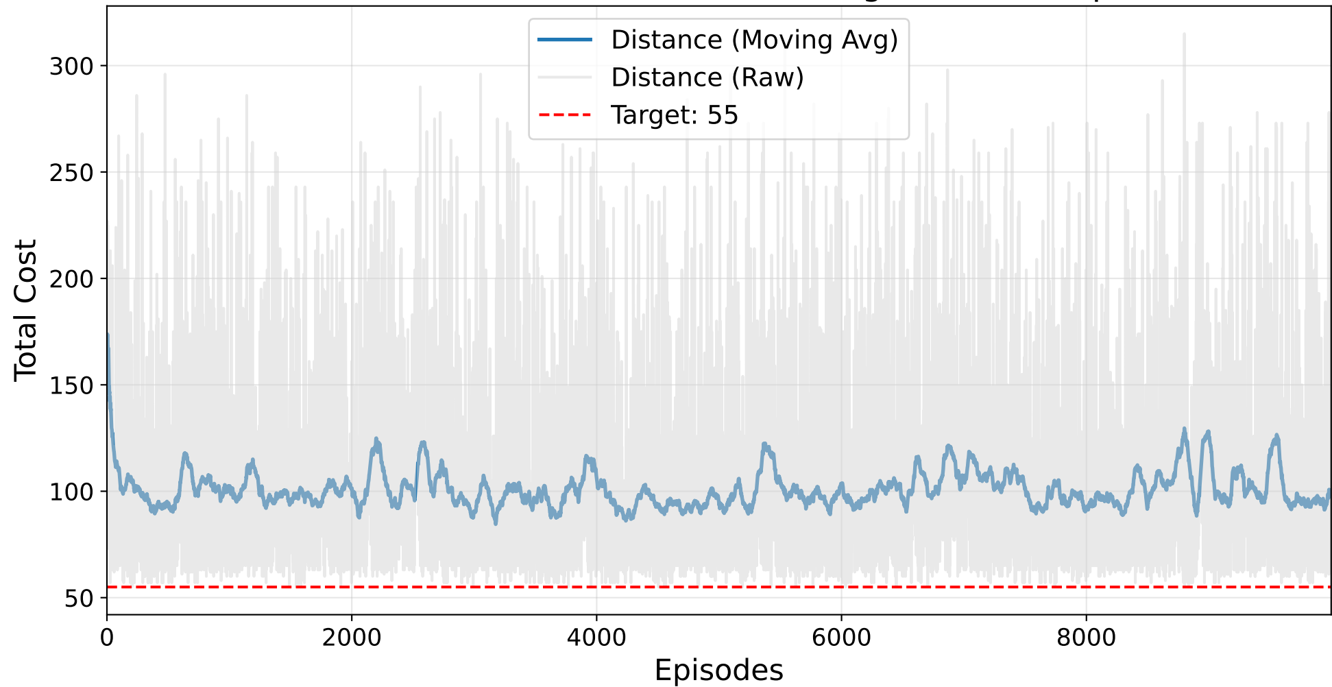
Final Masked AutoRL-SOP Training - br17.12.sop
